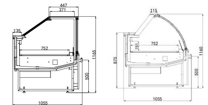
SCU Ivian Series Service Over Counter with Sliding Doors
