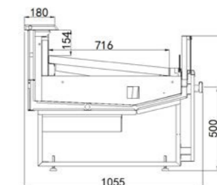
SCU Ivian Series Static-cooling Ice Counter
