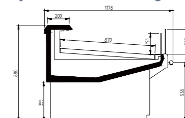
SGL Aries Boyar Series Static-cooling Ice Counter
