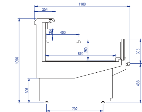
Medea Series Double Shelf Service Counter
