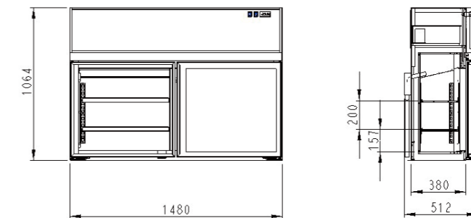
Ice cream Vertical Freezer
