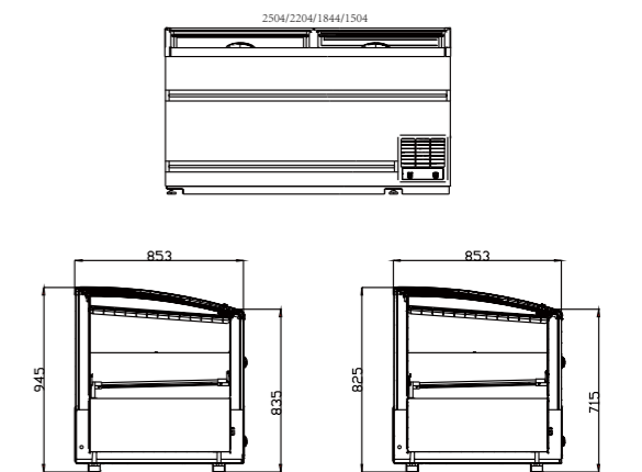
Adventer Plus Integral Chest Freezer (Plug-in)
